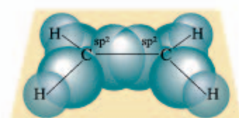
\sigma 键
